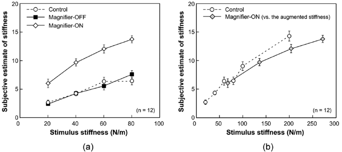
Figure 5. (a) Mean estimates of perceived stiffness. Error bars represent \pm 1 standard error. (b). Replot of the magnifier-ON and control data, including the stiffness tested only in dummy trials in the control condition. The magnifier-ON data were replotted versus the augmented stiffness produced by the force magnifier (i.e., 3.4\times stiffer as predicted from the augmented force).
