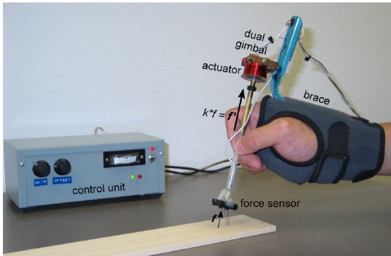
Figure 1. The force magnification device used in this study. The device uses a sensor to measure the force ( f ) between the tip and the target, which is amplified to produce f' = k*f ( k was set to 2.4 in this study) in the same direction on the handle using an actuator mounted on the back of the hand via a brace. The total force applied to the user's hand was thus ( F_{total} = f' + f ), producing a magnification of (1 + k) or 3.4 here.
