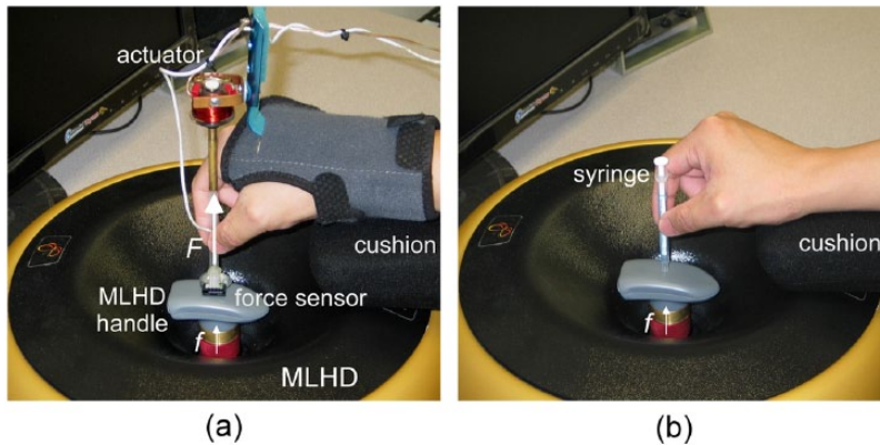
Figure 2. Illustration of the experimental setup. The user's perception of force was compared across the magnifier-ON/OFF conditions (a) and control condition (b). A magnetic levitation haptic device (MLHD) was used to produce the experimental stimuli.
